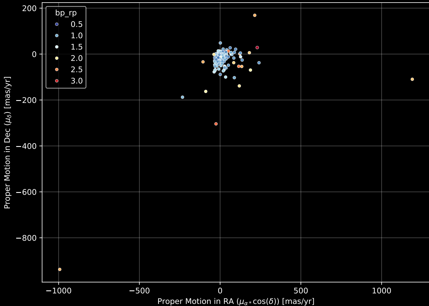
APOGEE DR17 Field: [087-58_MGA] Proper Motion Diagram (n= 209)
