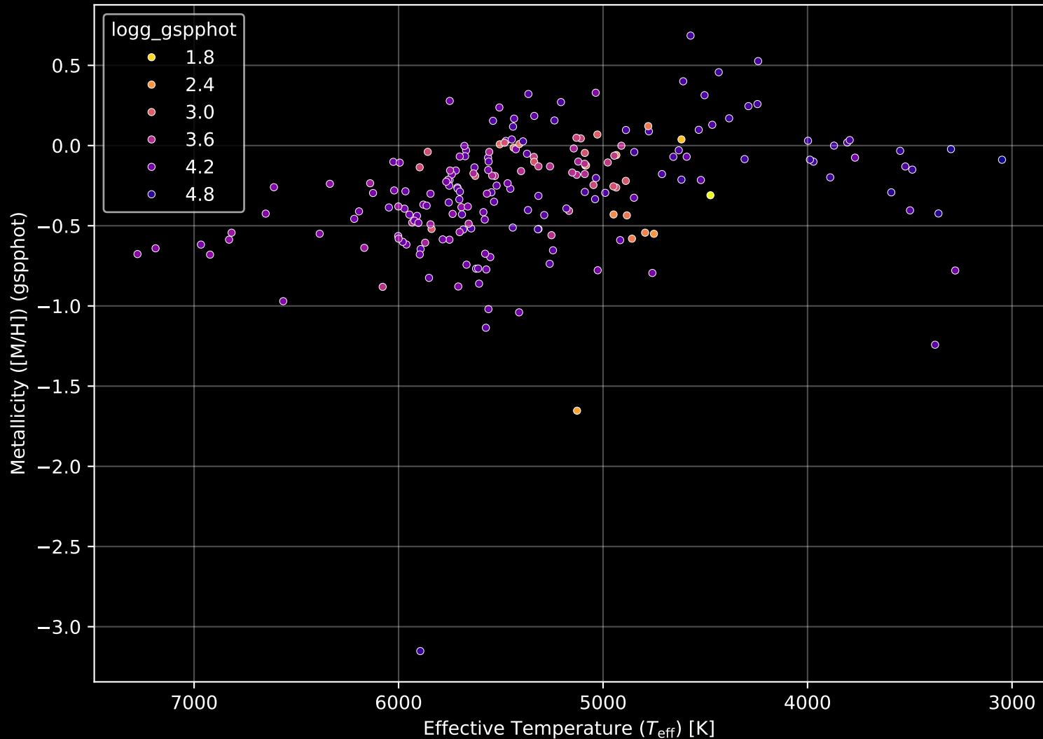
APOGEE DR17 Field: [087-58_MGA] Stellar Population Parameters (n= 209)
