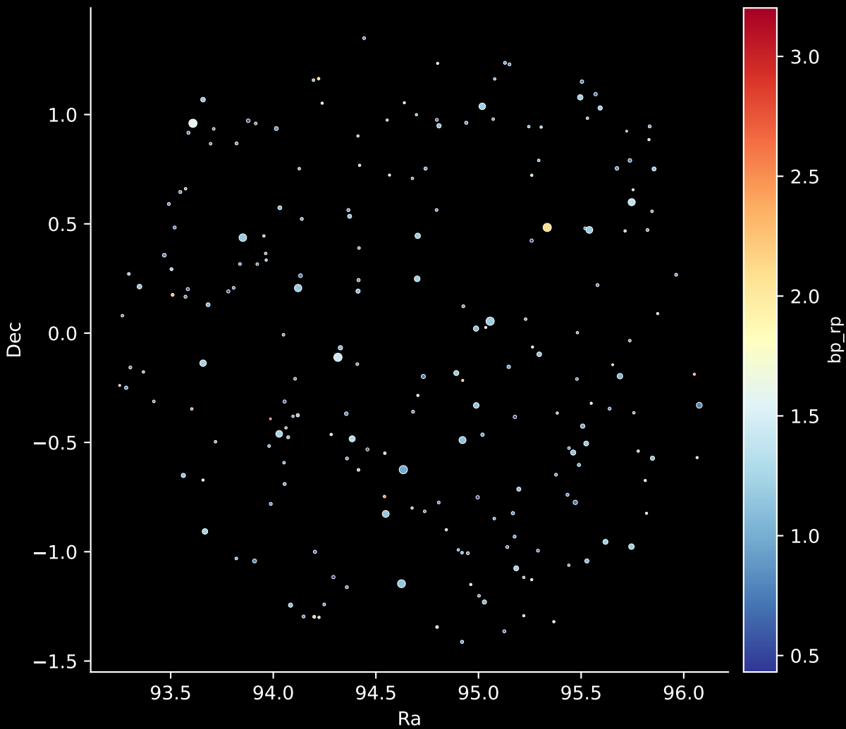
APOGEE DR17 Field: [087-58_MGA] Stars: 209
