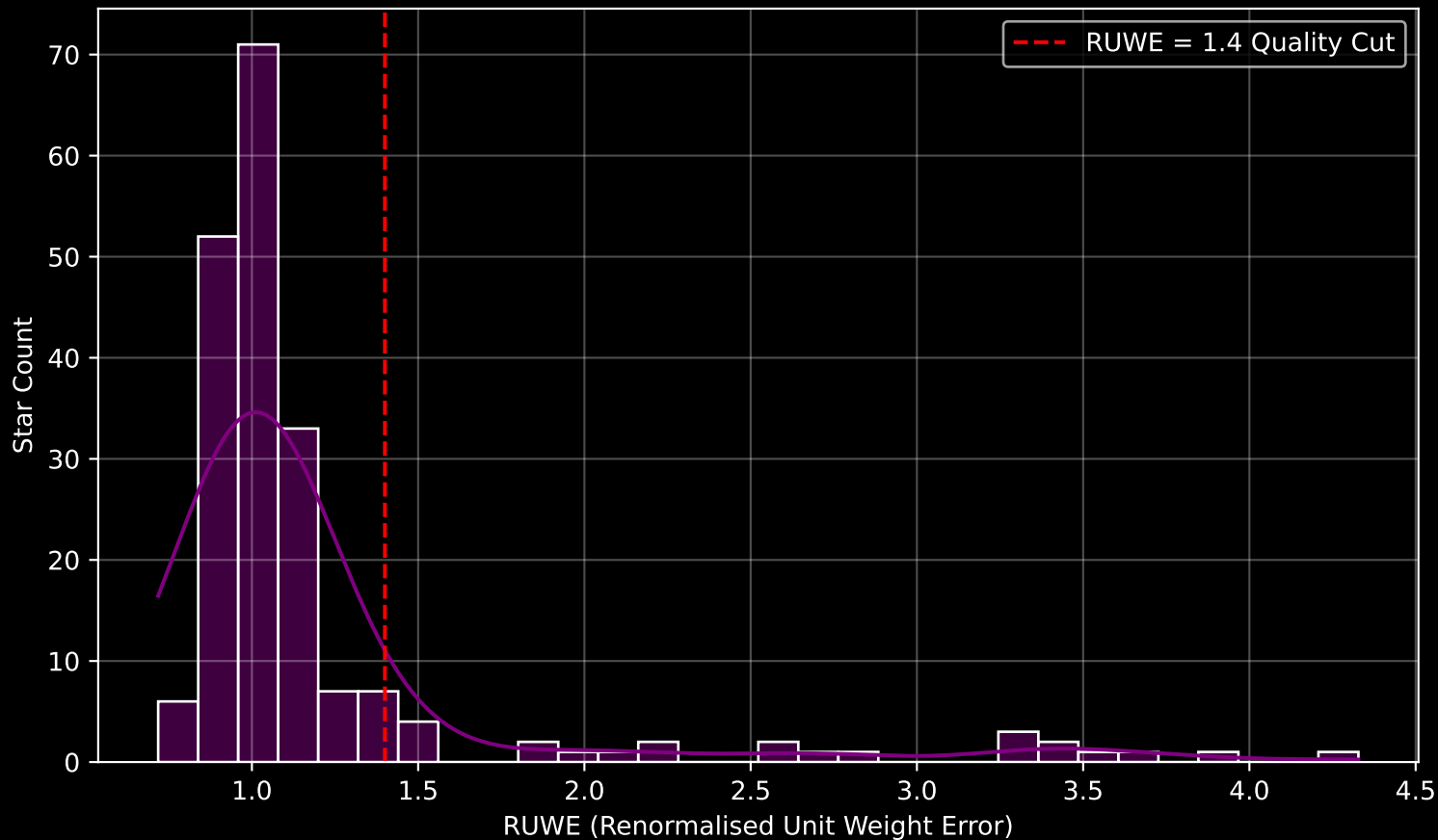
GAPOGEE DR17 Field [087-58_MGA] RUWE Distribution (n= 199)
