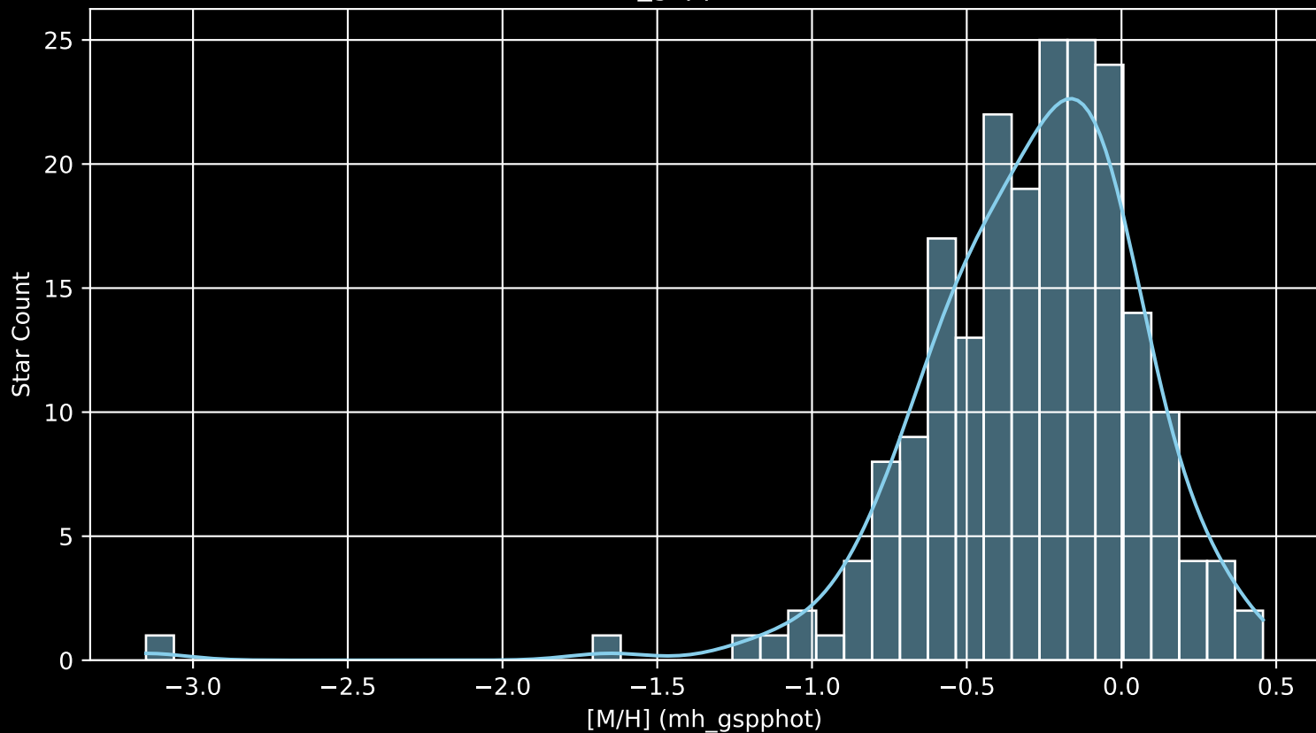
APOGEE DR17 Field: [087-58_MGA [M/H] (mh_gspphot) (n= 207)
