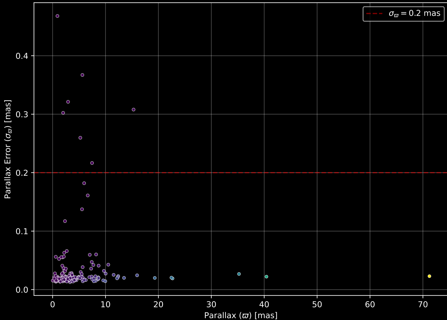
APOGEE DR17 Field: [087-58_MGA] Parallax Quality (n= 209)
