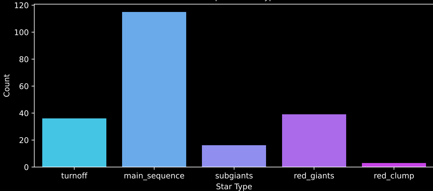
APOGEE DR17 Field: [087-58_MGA] Count plot of Star Type
